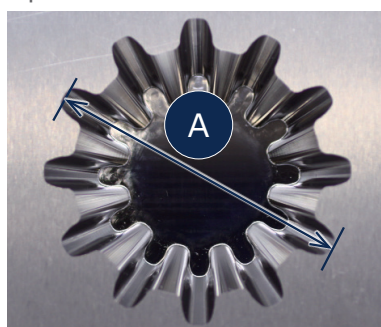
歯先円直径 Tip circle diameter
