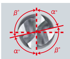
不等分割 Unequal Flute Spacing
